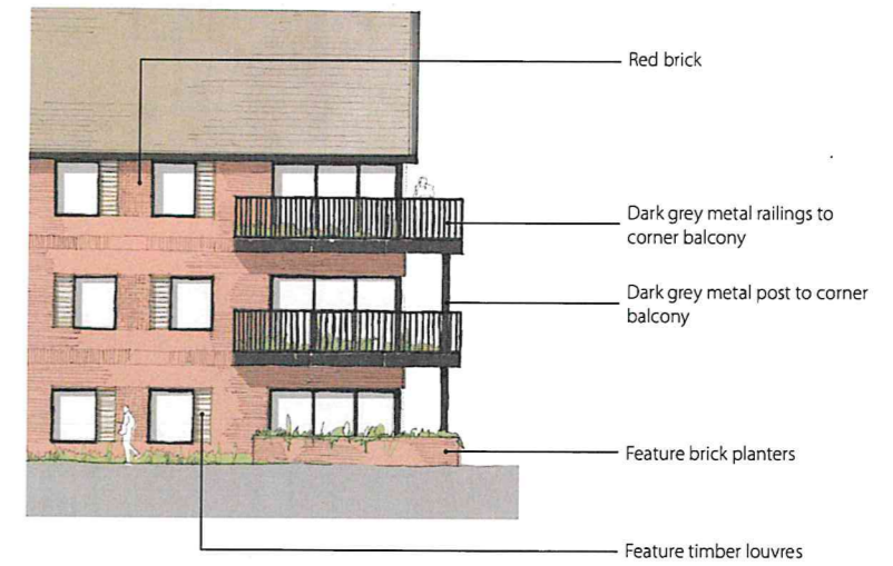
Bay study- illustrating architectural style
