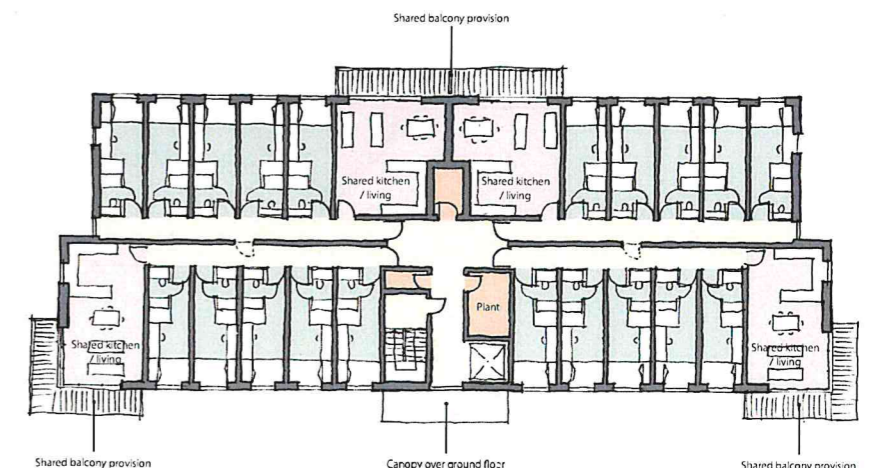
Second floor plan (20 beds)
