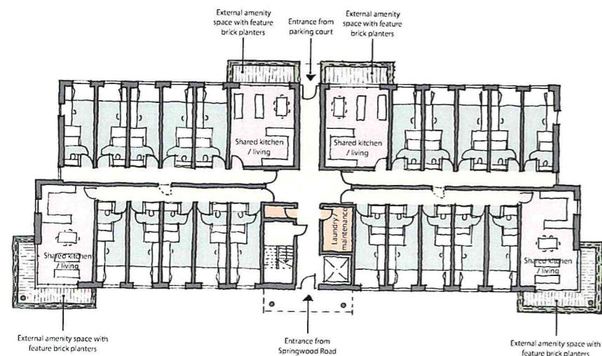
Ground floor plan (20 beds)
